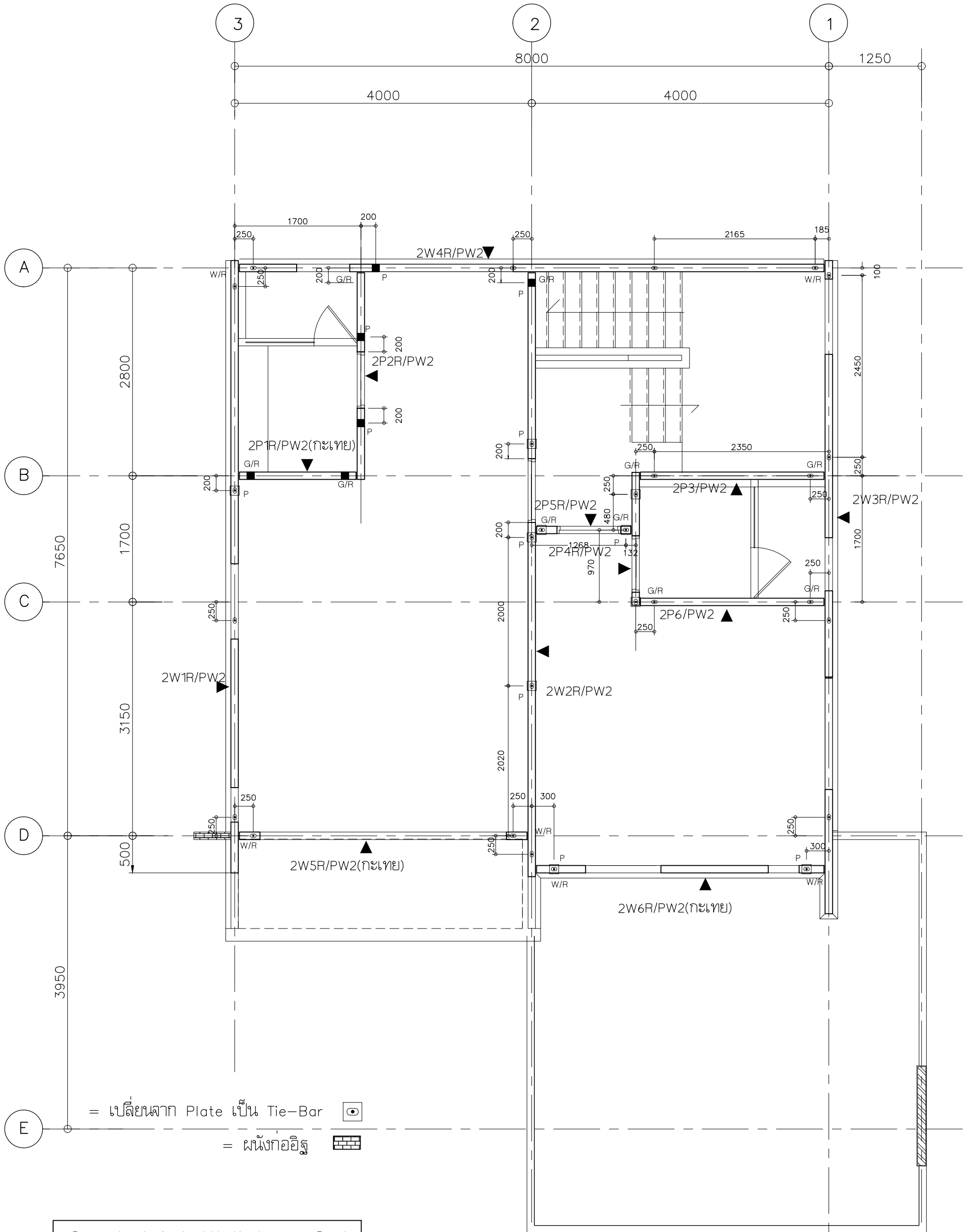
2 nd Joint Wall Lay-Out
